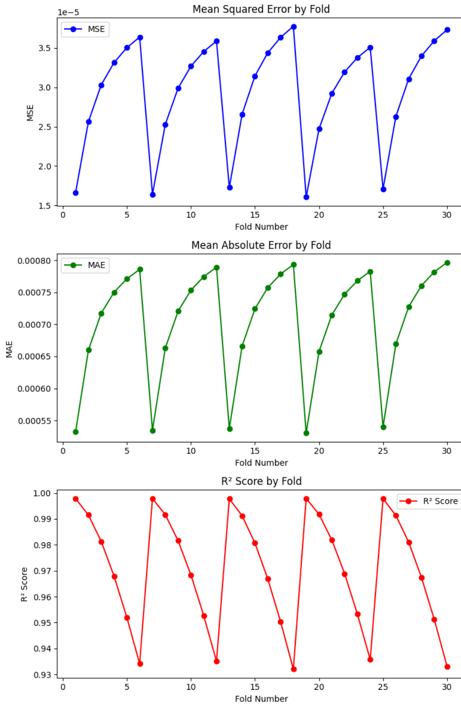
Figure 15: k-fold Cross-Validation per Metric plots (MSE, MAE & R²)
