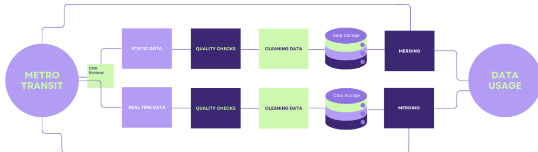
Figure 11: Pipeline Overview Diagram
