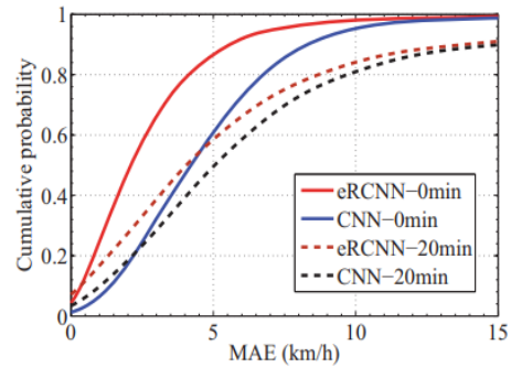
Figure 2: The diagram shows that adding independent error-feedback neurons to eRCNN improves its ability to forecast traffic speeds with sudden variations. Given that eRCNN's absolute prediction error is lower than CNN's, the error-feedback system has significantly improved, particularly in handling traffic
