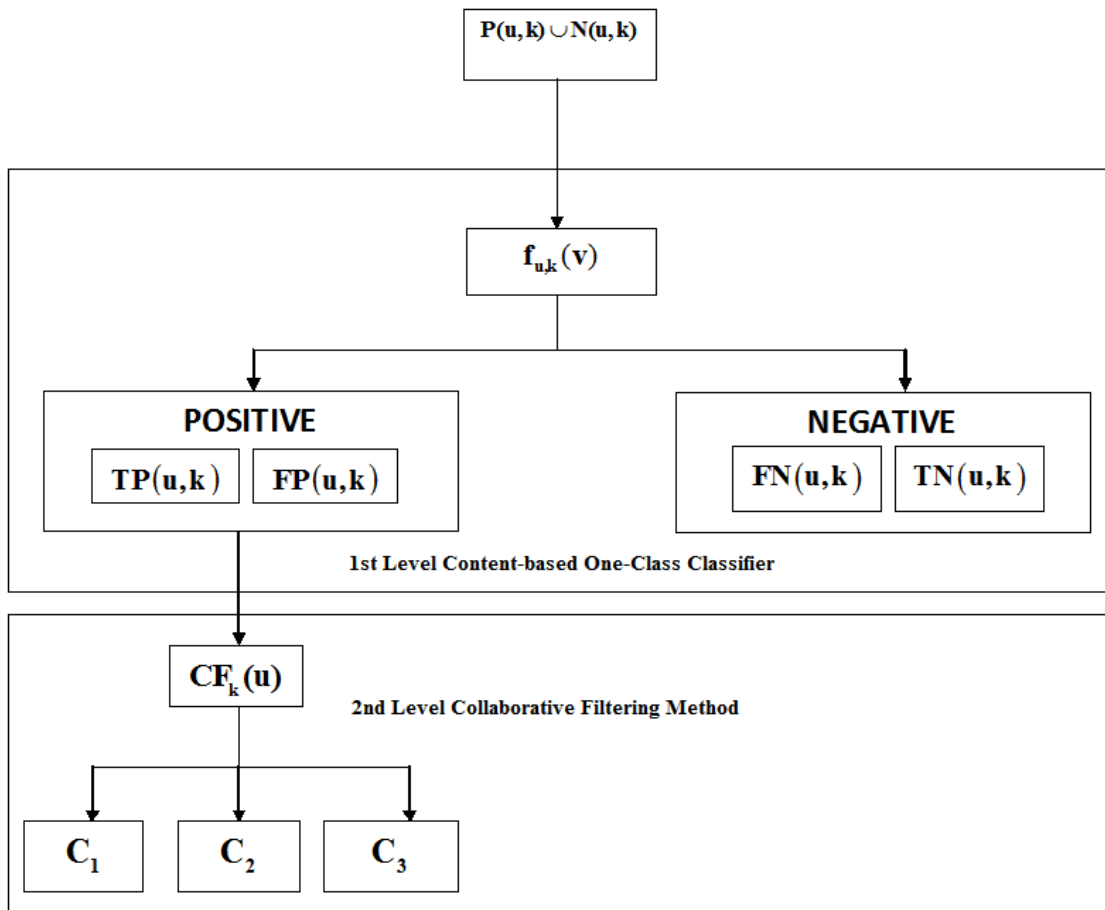
Figure 6-2: Cascade Hybrid Recommender.
