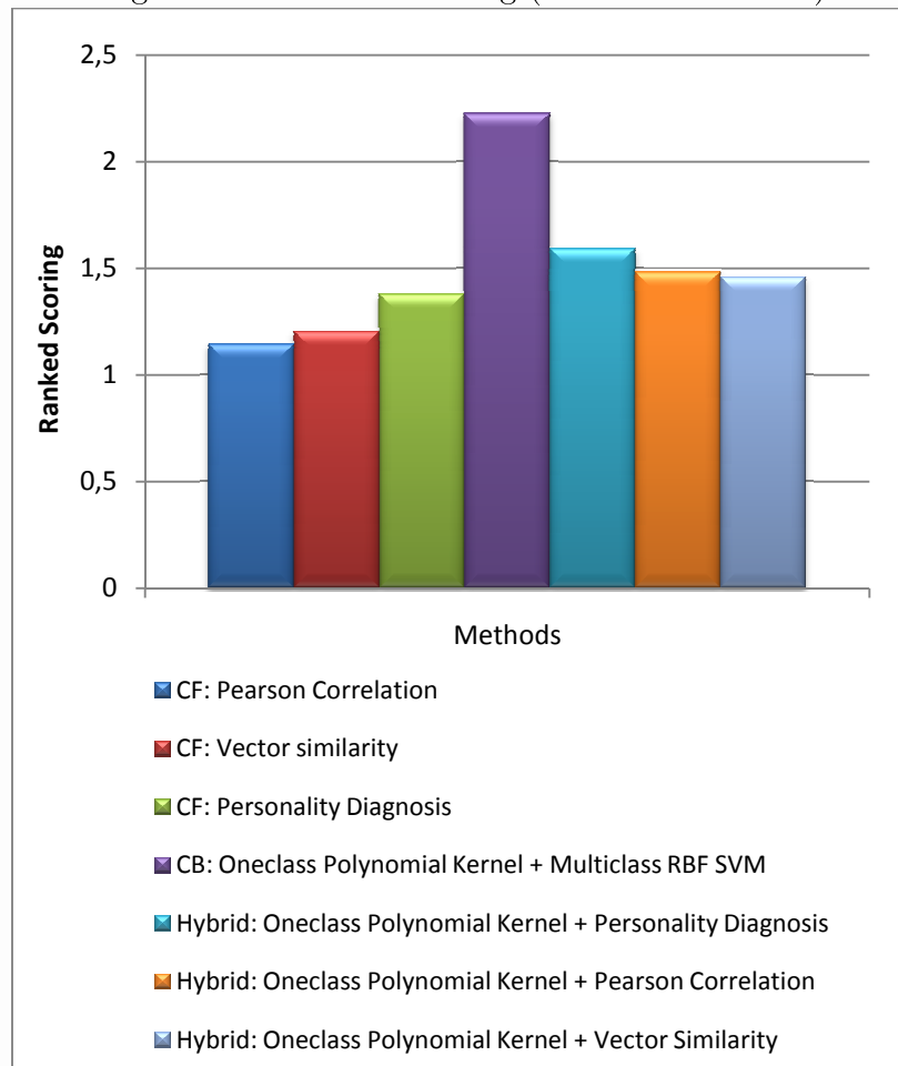
Figure 7-6: Ranked Scoring (Mean for all users)
