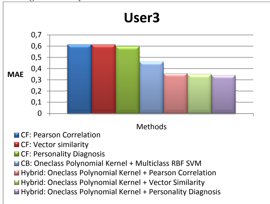
Figure 7-3: Hybrid Recommender is the best for User3
