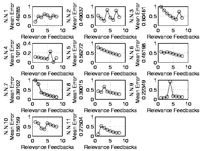
Figure 5-4: Typical User Behavior I.
