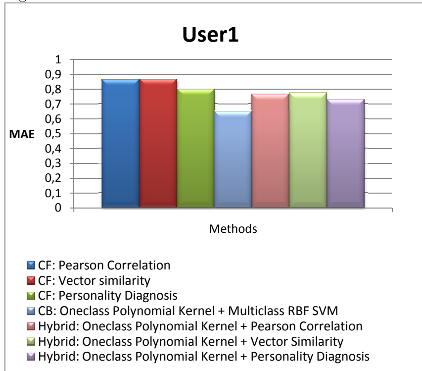
Figure 7-1: Content-based Recommender is the best for User 1
