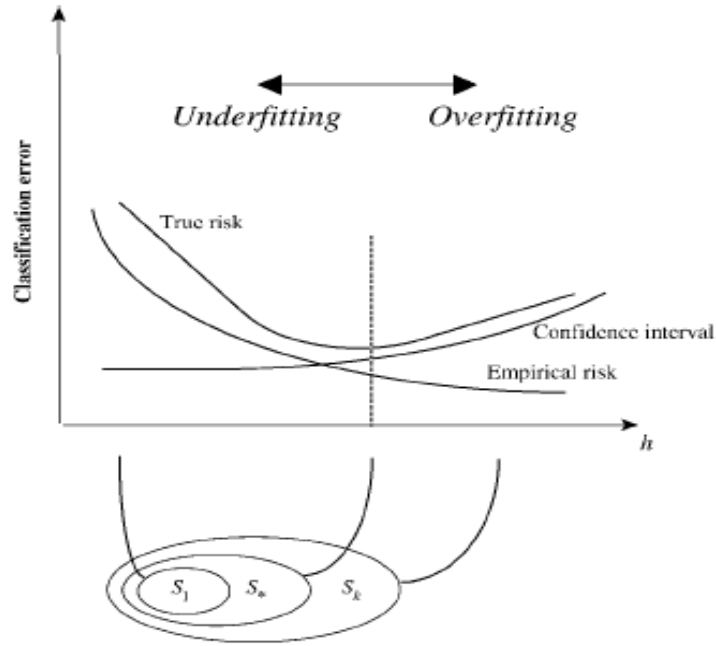
Figure 3-3: Upper bound on Expected True Risk R(a) and Empirical Risk R_{emp}(a) as a function of VC dimension h
