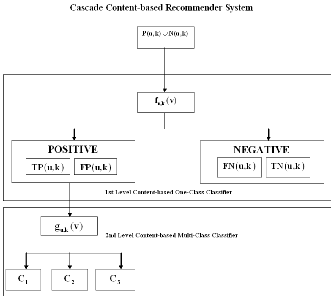
Figure 6-1: Cascade Content-based Recommender.
