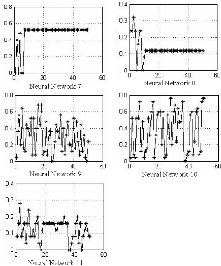
Figure 5-7: Precision of Neural Networks 7-11 for the one user.
