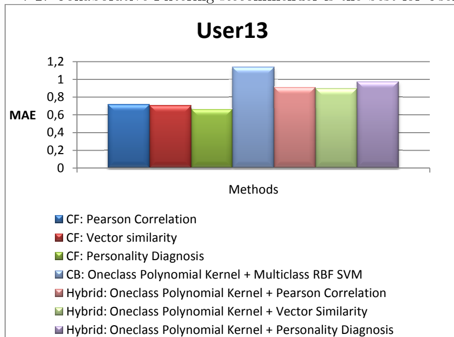
Figure 7-2: Collaborative Filtering Recommender is the best for User 13
