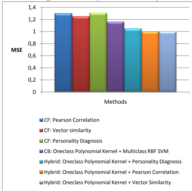
Figure 7-5: MSE (Mean for all users)
