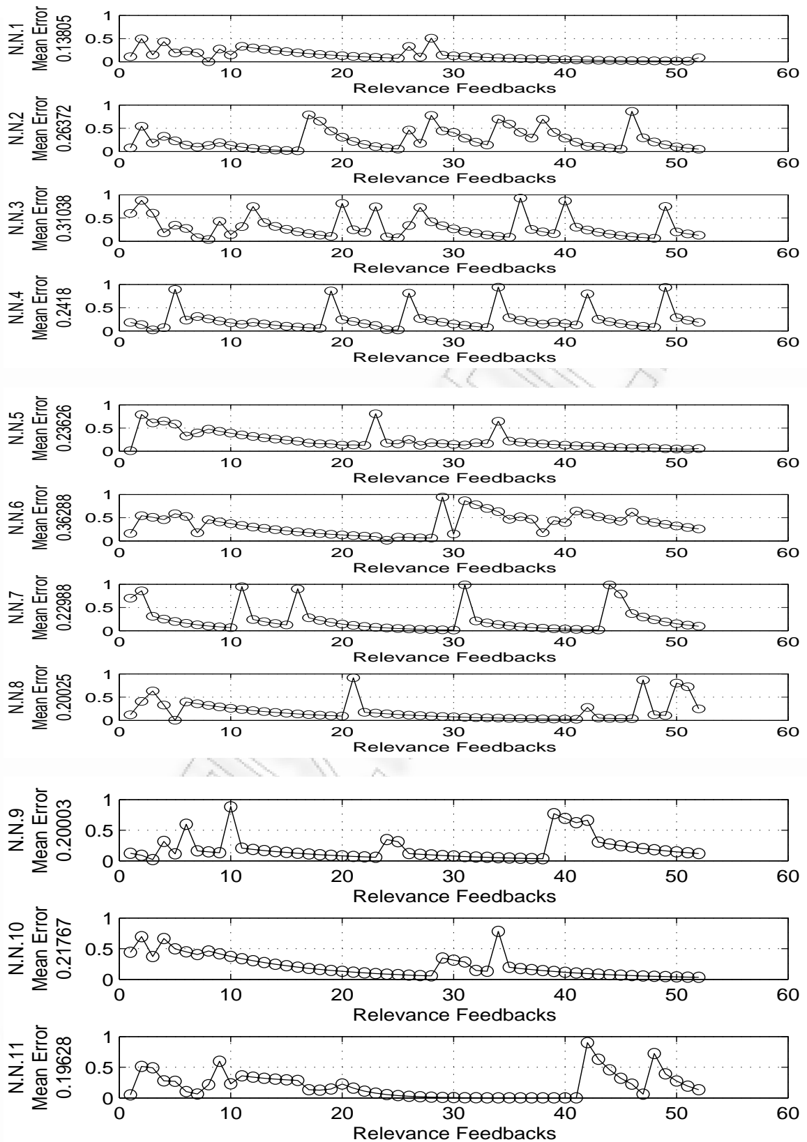
Figure 5-11: Error Rate Convergence.
