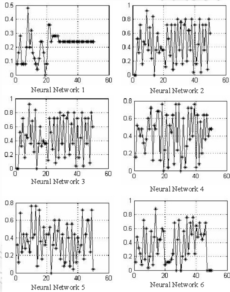
Figure 5-6: Precision of Neural Networks 1-6 for the one user.
