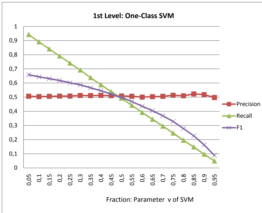
Figure 7-11: One Class SVM (Precision, Recall, F1)
