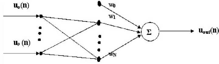
Figure 5-2: RBFN Architecture.
