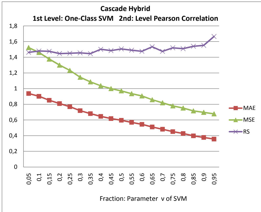
Figure 7-9: Hybrid Recommender 2nd Level Pearson Correlation: Fraction Analysis.
