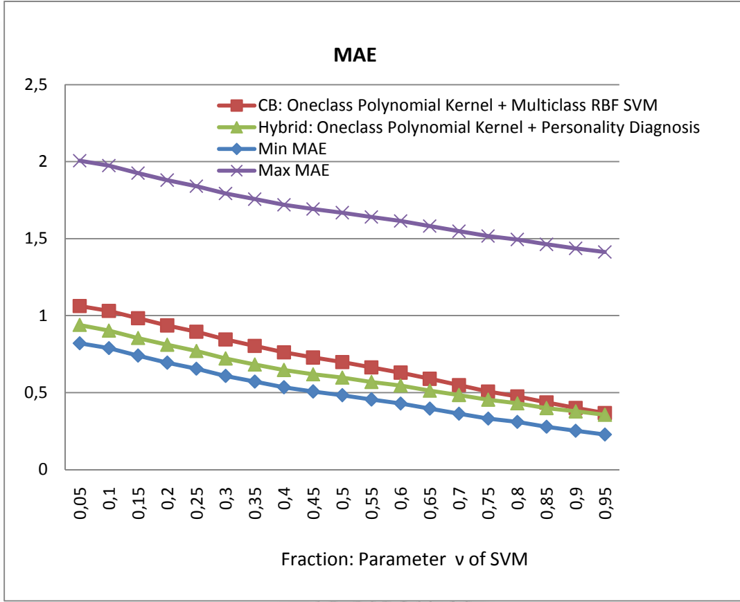
Figure 7-7: MAE Boundaries for One-Class SVM.
