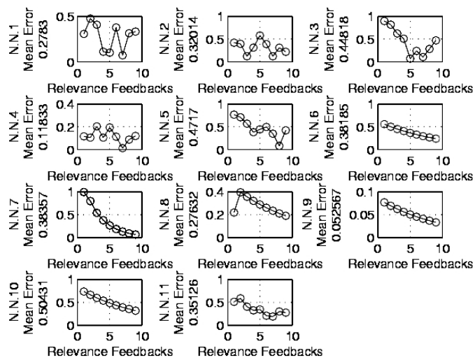
Figure 5-5: Typical User Behavior II.
