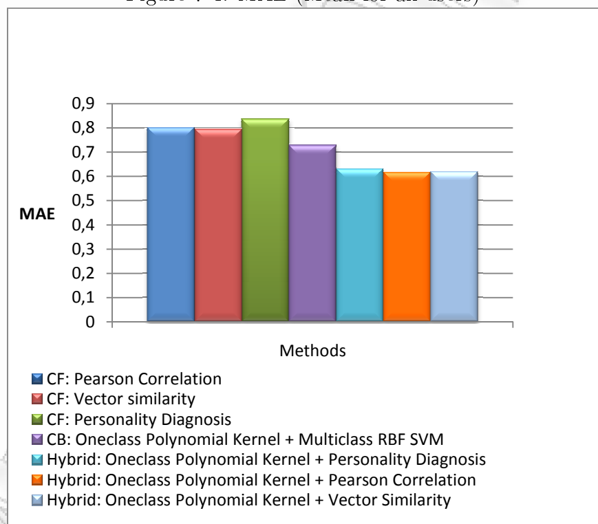
Figure 7-4: MAE (Mean for all users)
