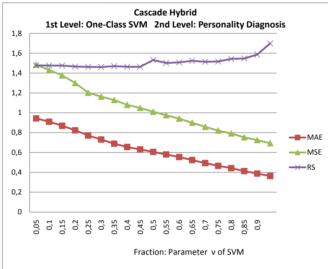
Figure 7-8: Hybrid Recommender 2nd Level Personality Diagnosis: Fraction Analysis.
