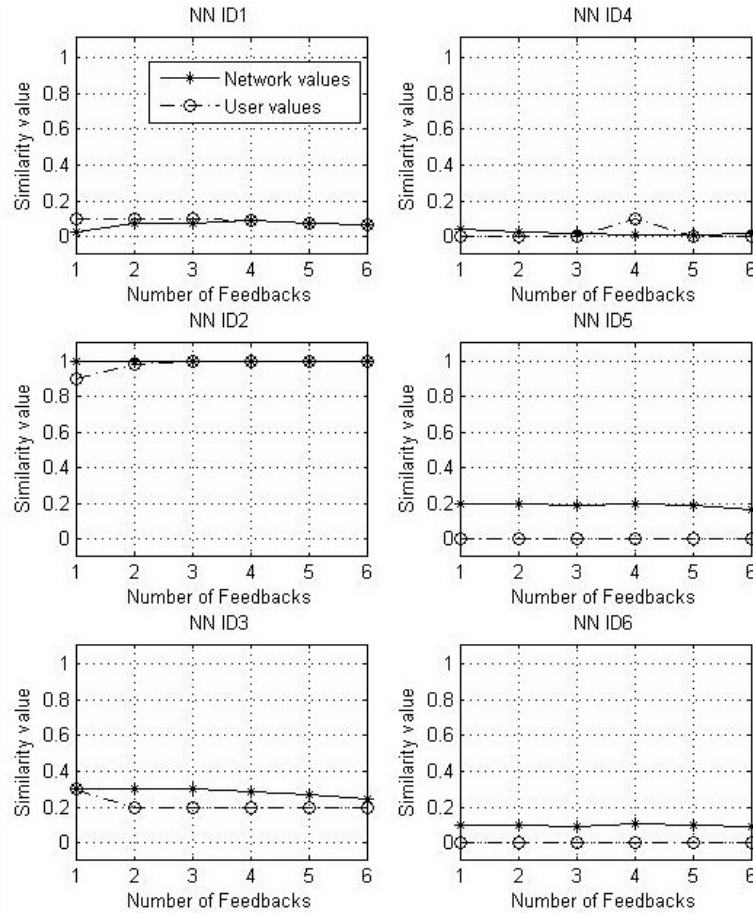
Figure 5-8: Comparison between network-estimated and user-supplied similarity values.
