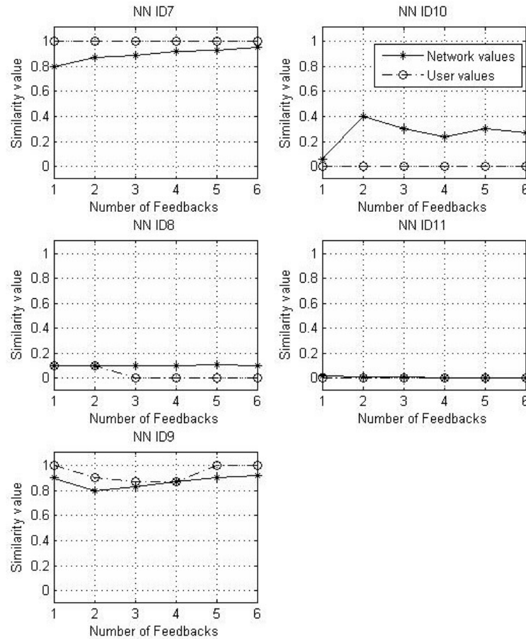
Figure 5-9: Comparison between network-estimated and user-supplied similarity values.
