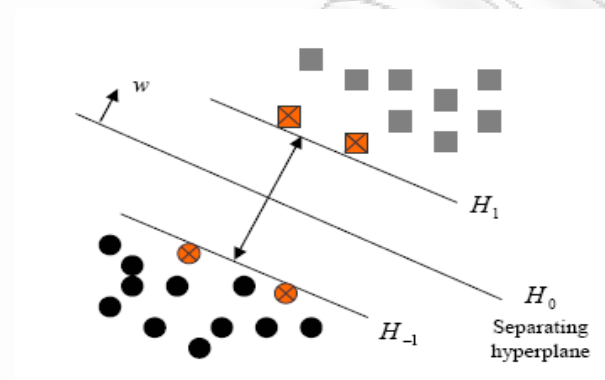
Figure 3-4: Two class classification. Support vectors are indicated with crosses
