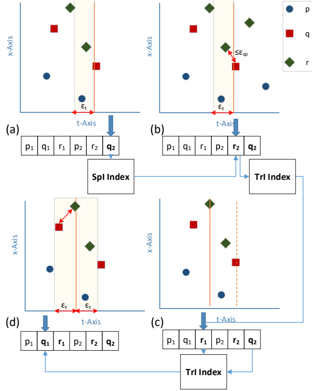
Figure 6.8: Example of \text{TRJPlaneSweep}^I .
