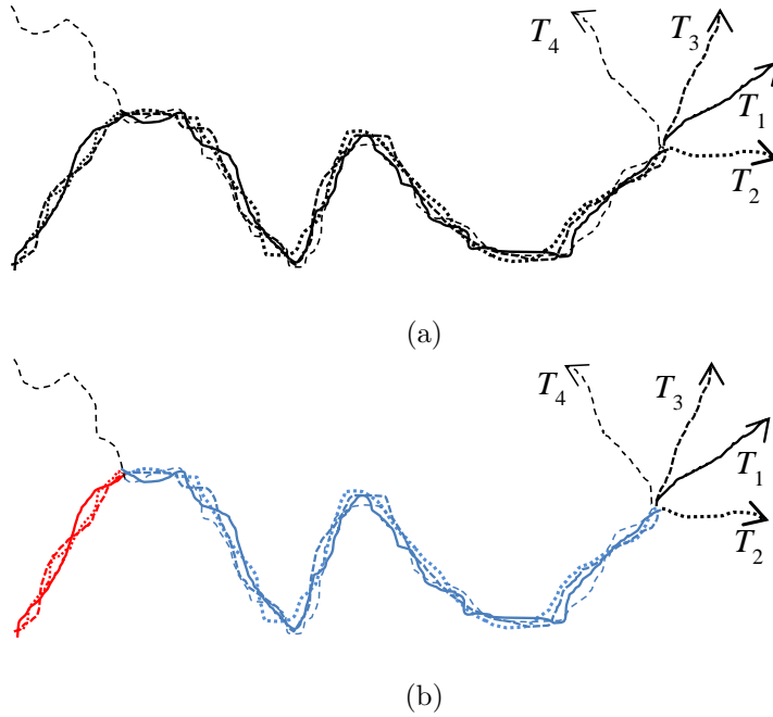
Figure 3.1: (a) a set of 4 trajectories; (b) the set split in 2 clusters (in red and blue) and 5 outliers (in black).
