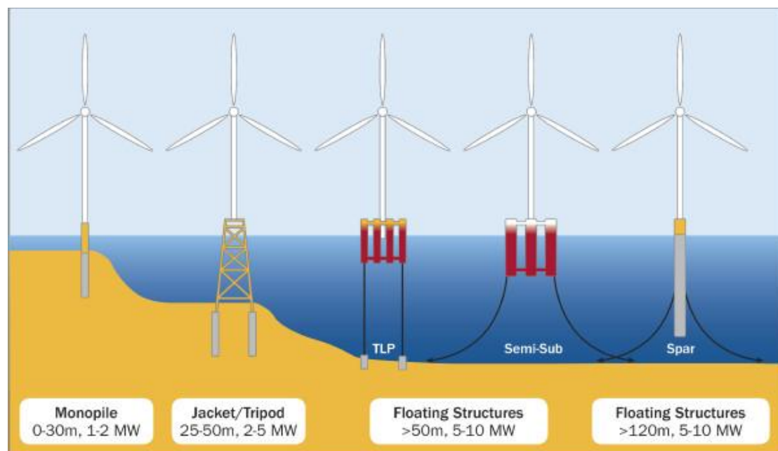
Figure 11: Types of Foundations (Research Gate)
